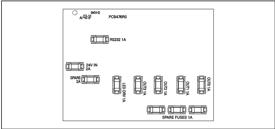
Figure 2. Fuse Locations
